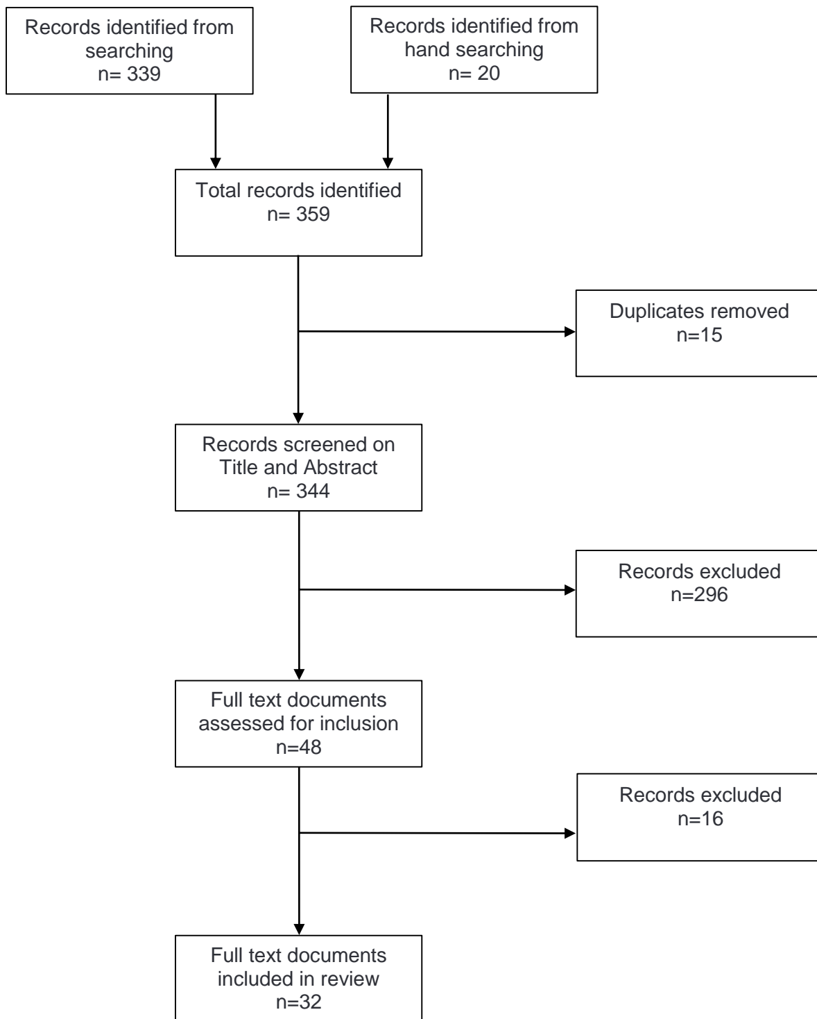
Figure A1: Literature search flowchart
